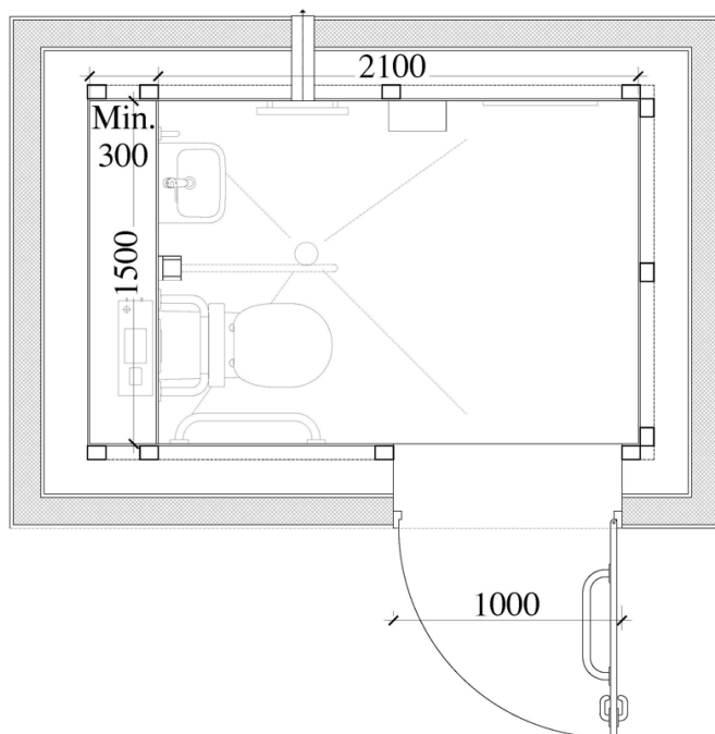
Compact External
